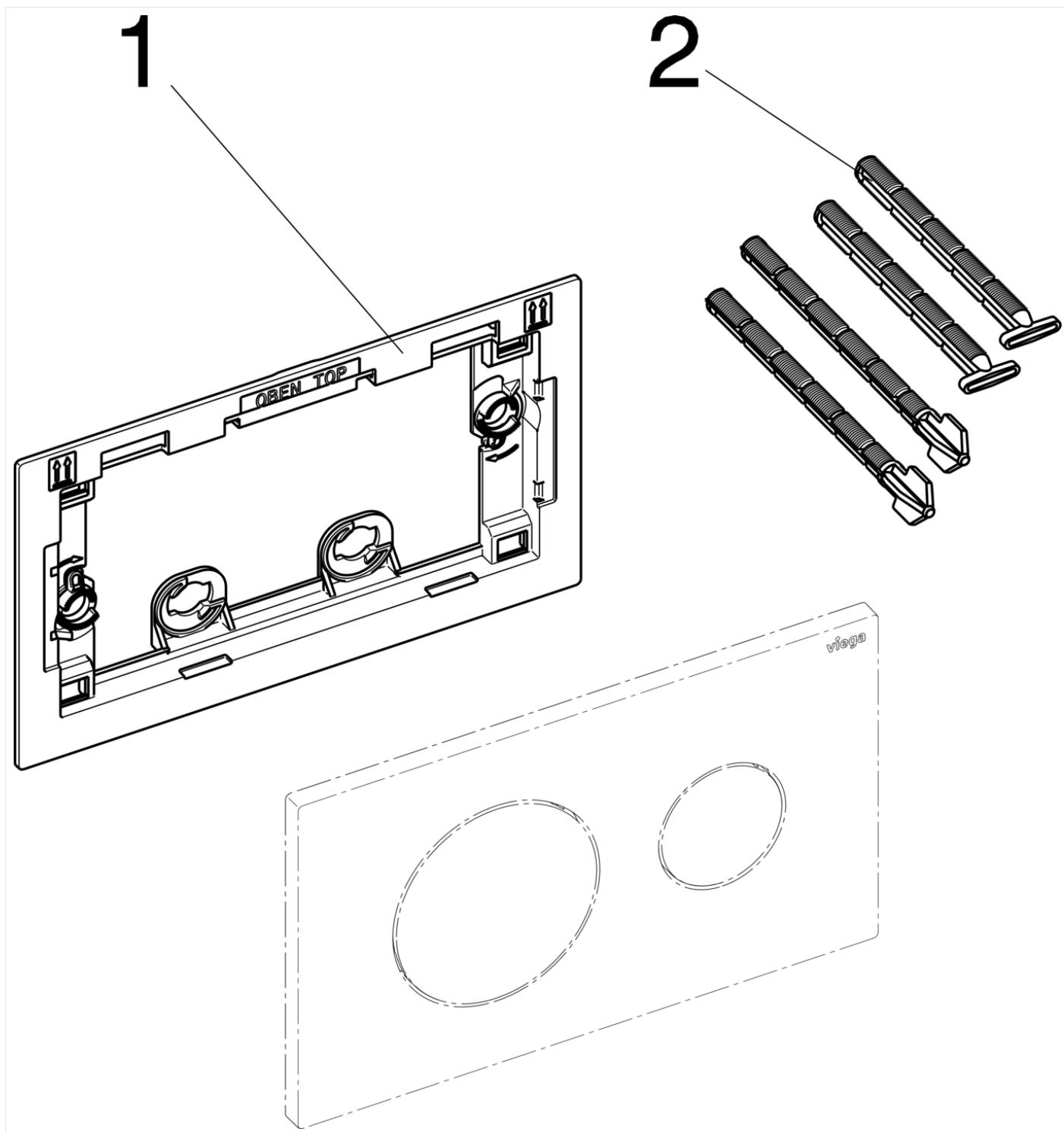
1. WC base frame Model 8580.22 (786373)
